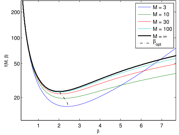
Fig. 1. Values of f(M, \beta) that governs the CRB as a function of the observation duration T = \beta/\alpha . M is the number of samples in the interval [0, T] , \alpha is the decay time of the sinusoid.
